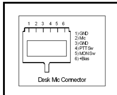
FIGURE 1. Desk Mic Connector Pin Outs
