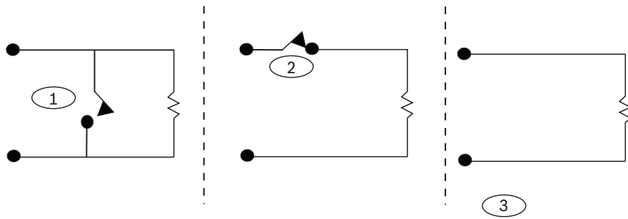
Figure 16.1: Single EOL resistor option
